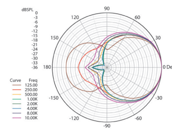
Supercardioid
