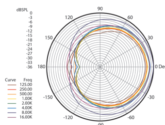
Cardioid
